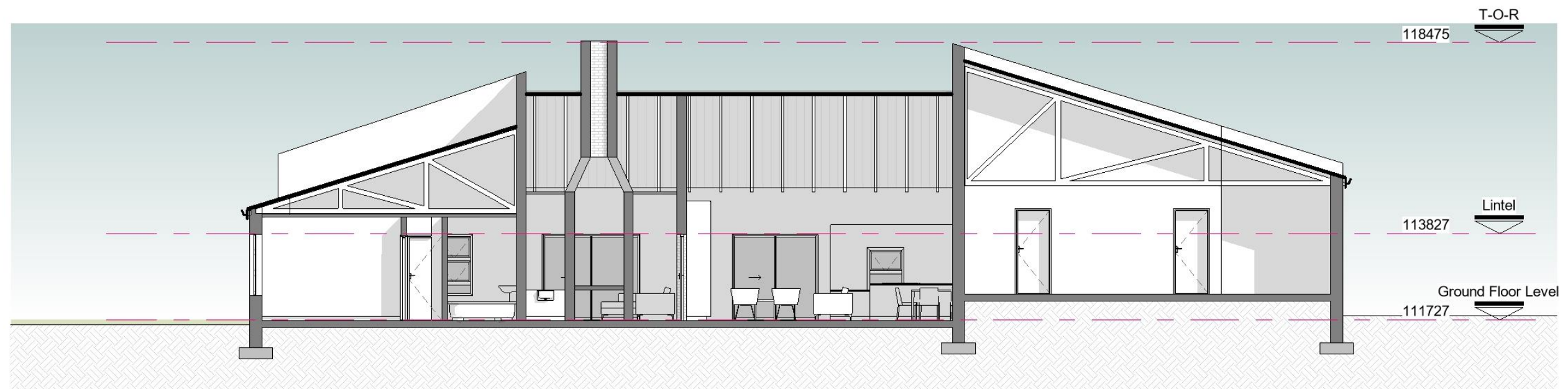
5-2 Section BB
