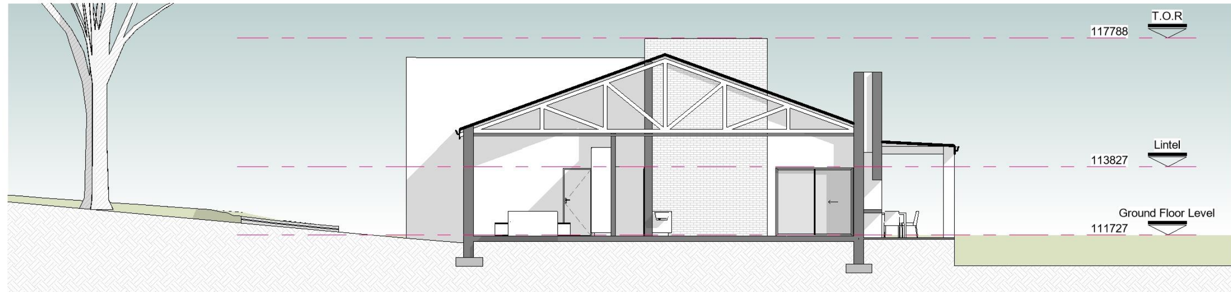
5-2 Section AA
