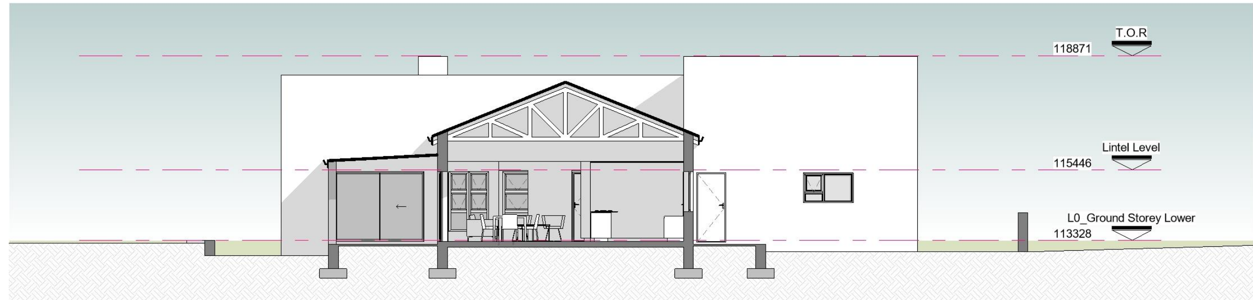
5-2 Section AA
