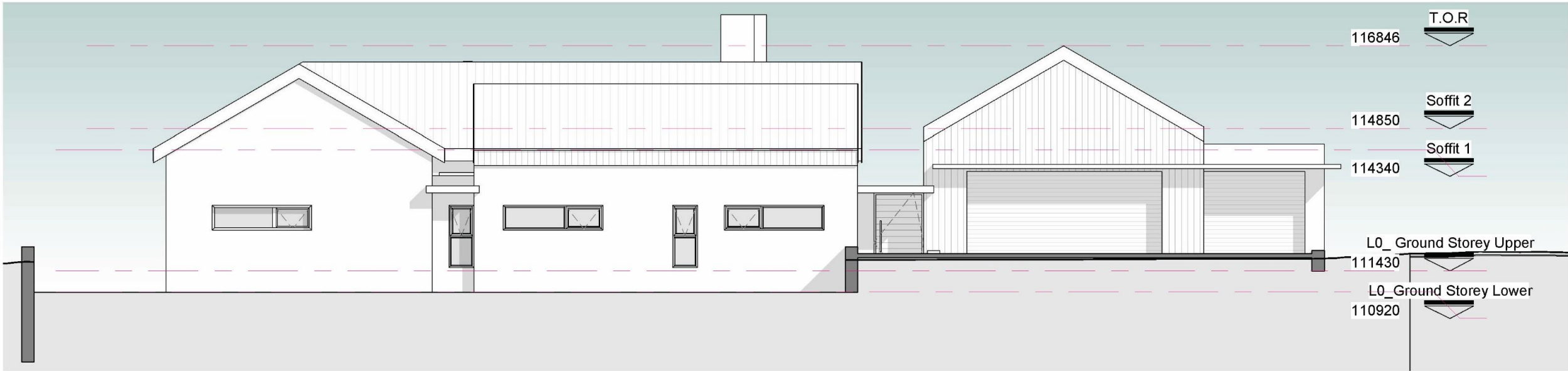
4-2 West Elevation 1 : 100
